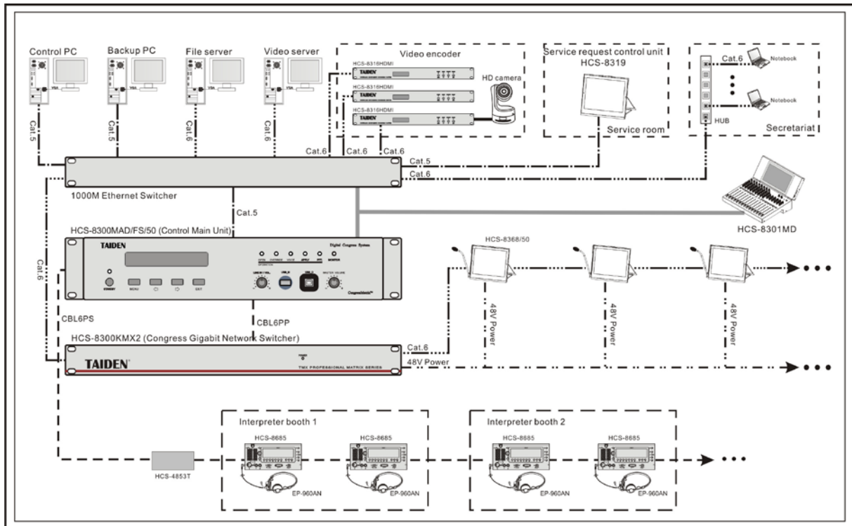
Figure 4a HCS-8368/50 Series G3 Paperless Multimedia Congress System connection diagram
